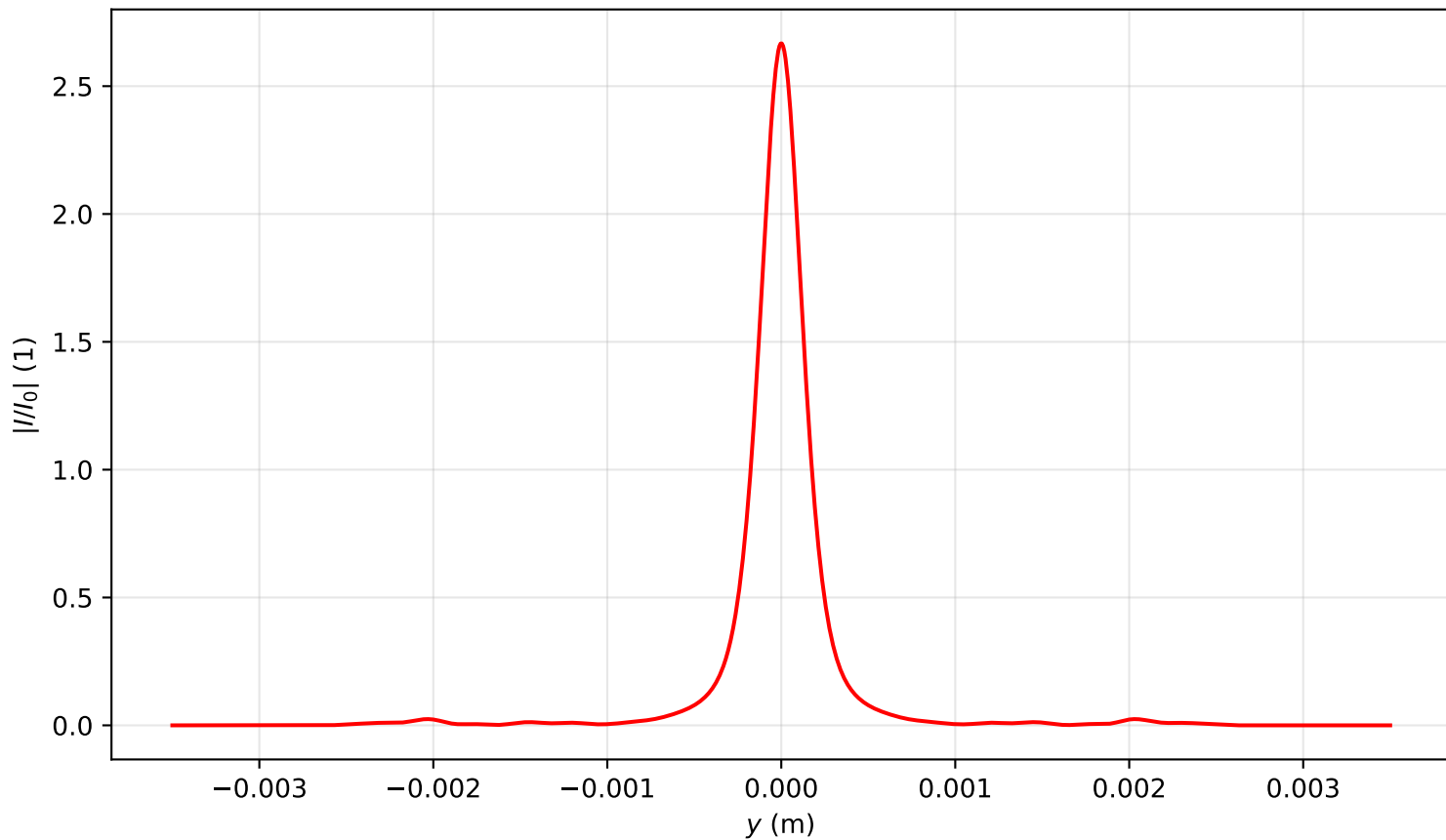
Intensity profile I(x = 0, y, z = 3.344)/I_0 , \text{Pin}=2.5\text{Pcr} , artificial time
